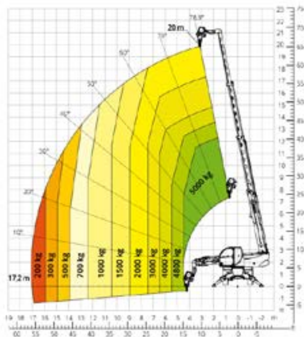
Load chart with WINCH 5,000 kg ATT - 02 - 019
