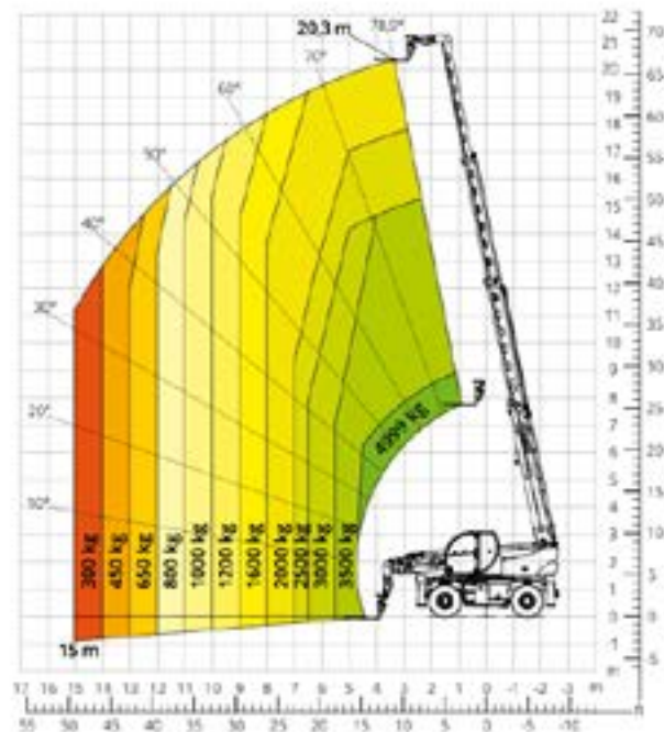
Load chart FRONT ATTACHMENT ON TYRES ATT - 03 - 001
