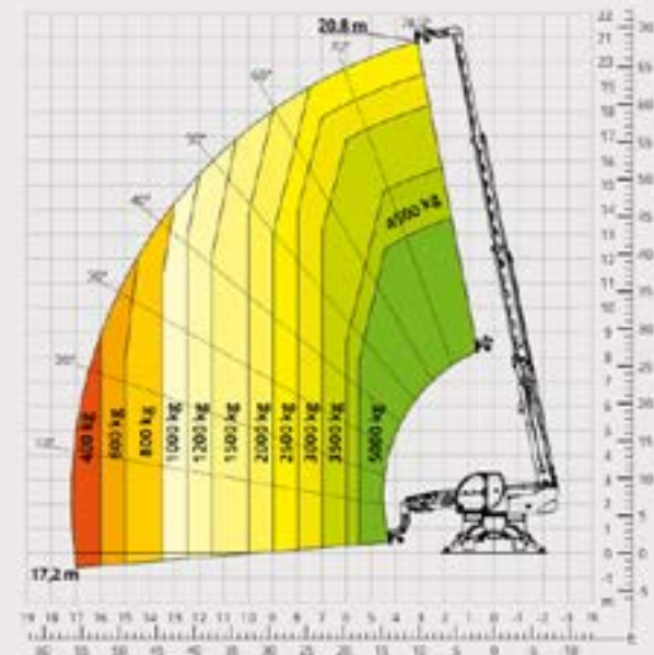
Load chart with HOOK, 5,000 kg ATT - 05 - 014
